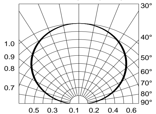
Fig.6-Radiation Diagram
