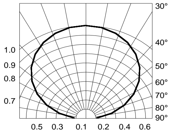
Fig.6-Radiation Diagram
