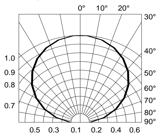
Fig.6-Radiation Diagram Ta=25°C
