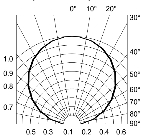
Fig.6-Radiation Diagram
