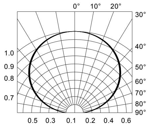
Fig.6-Radiation Diagram Ta=25°C
