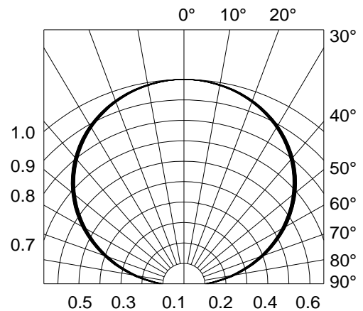
Fig.6-Radiation Diagram Ta=25°C
