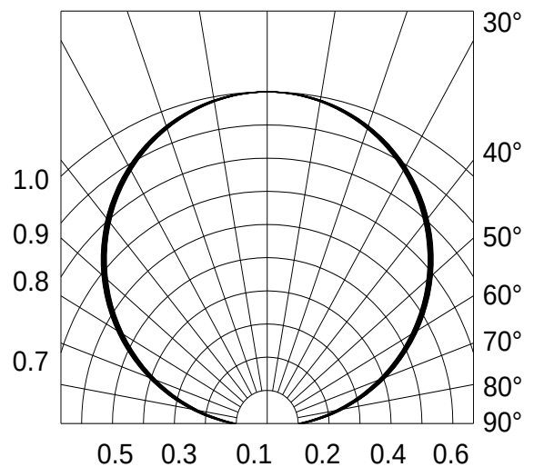
Fig.6-Radiation Diagram Ta=25°C 0° 10° 20°
