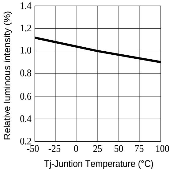
Fig.3-Relative Luminous Intensity vs.Juntn Temperature
