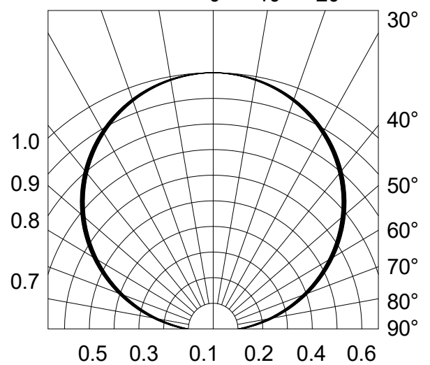
Fig.6-Radiation Diagram Ta=25°C
