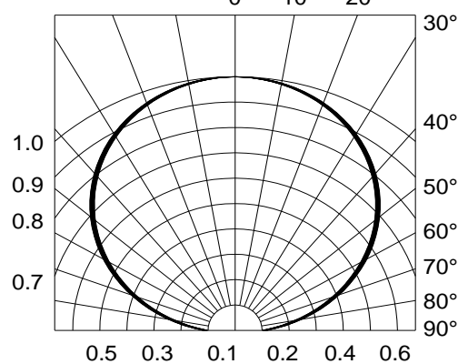
Fig.6-Radiation Diagram
