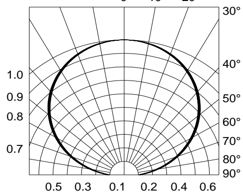
Fig.6-Radiation Diagram
