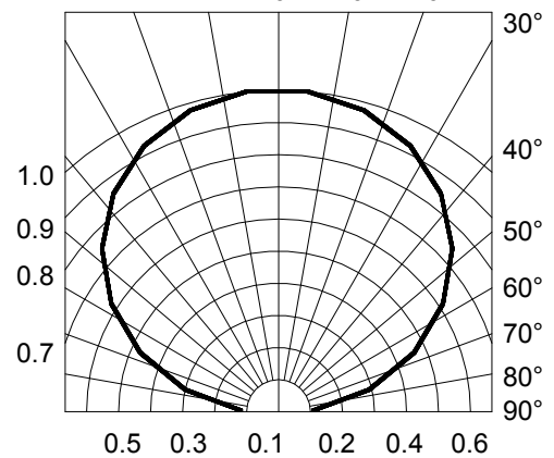
Fig.6-Radiation Diagram Ta=25°C
