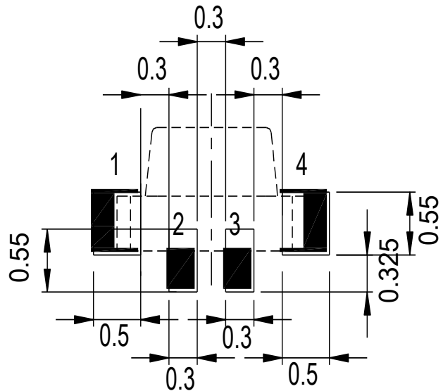
Recommended Solder Pad
