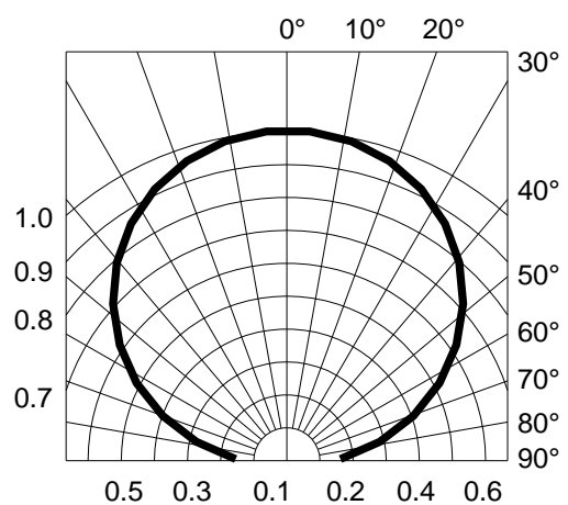
Fig.6-Radiation Diagram Ta=25°C
