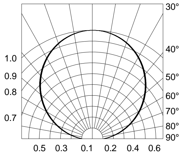
Fig.6-Radiation Diagram T_a=25^\circ\text{C} 0° 10° 20°
