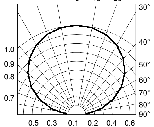
Fig.6-Radiation Diagram T_a=25^\circ\text{C}
