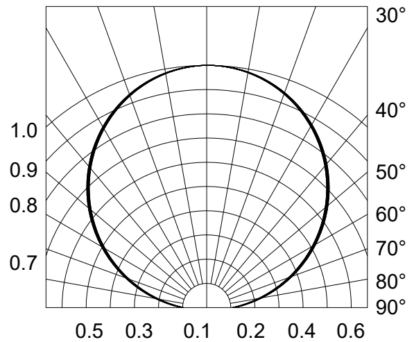
Fig.6-Radiation Diagram T_a=25^{\circ}\text{C} 0^{\circ} 10^{\circ} 20^{\circ}
