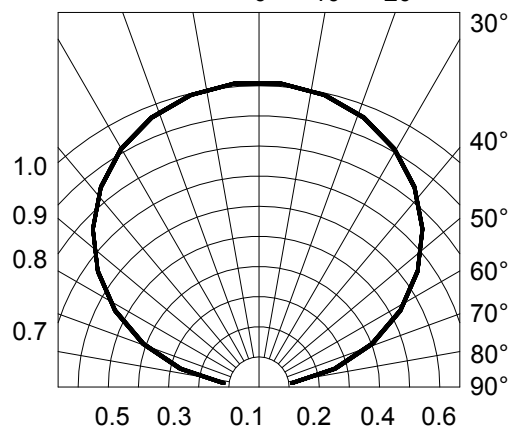
Fig.6-Radiation Diagram
