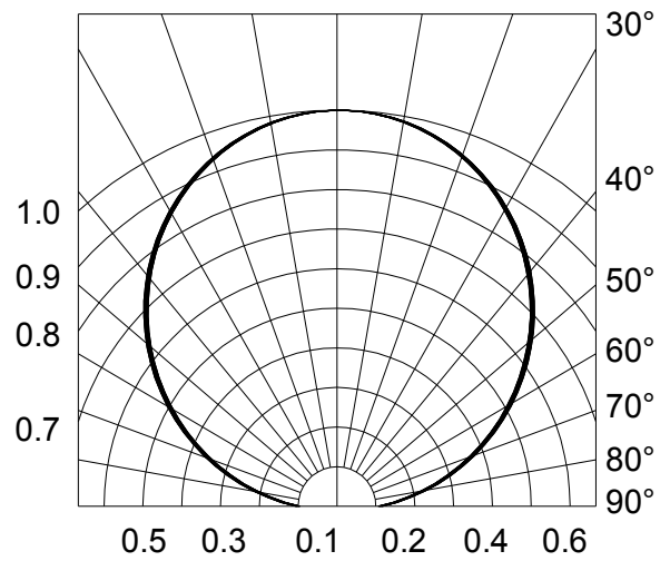
Fig.6-Radiation Diagram Ta=25°C
