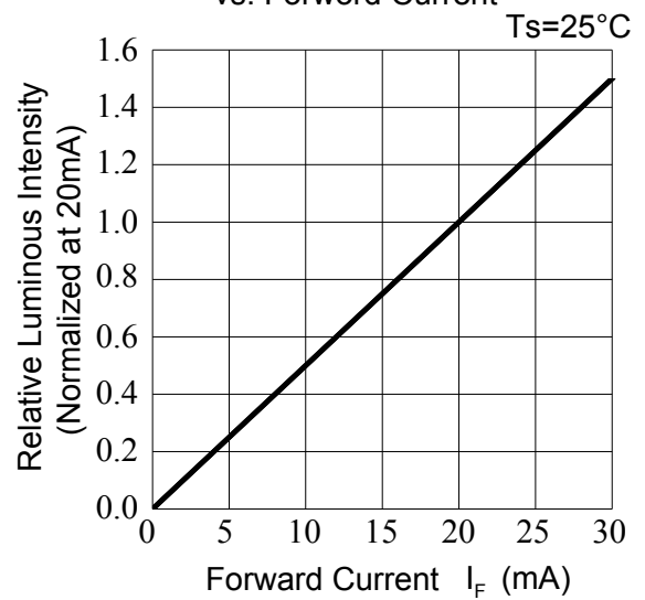
Fig.2-Relative Luminous Intensity vs. Forward Current Ts=25°C
