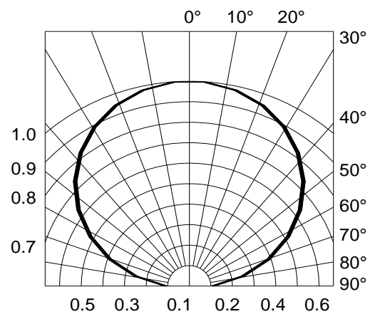
Fig.6-Radiation Diagram Ta=25°C
