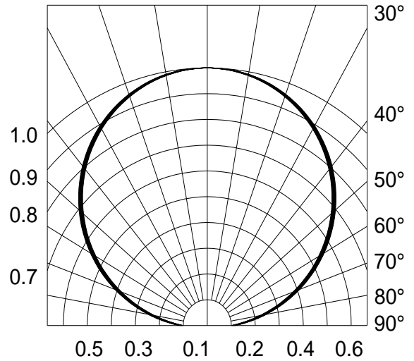
Fig.6-Radiation Diagram Ta=25°C 0° 10° 20°
