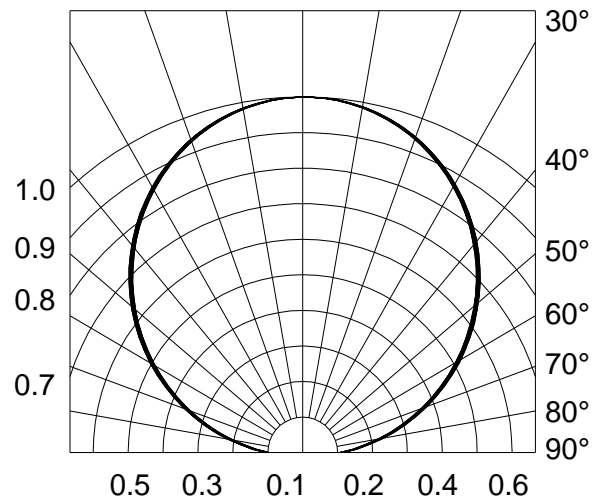
Fig.6-Radiation Diagram Ta=25°C
