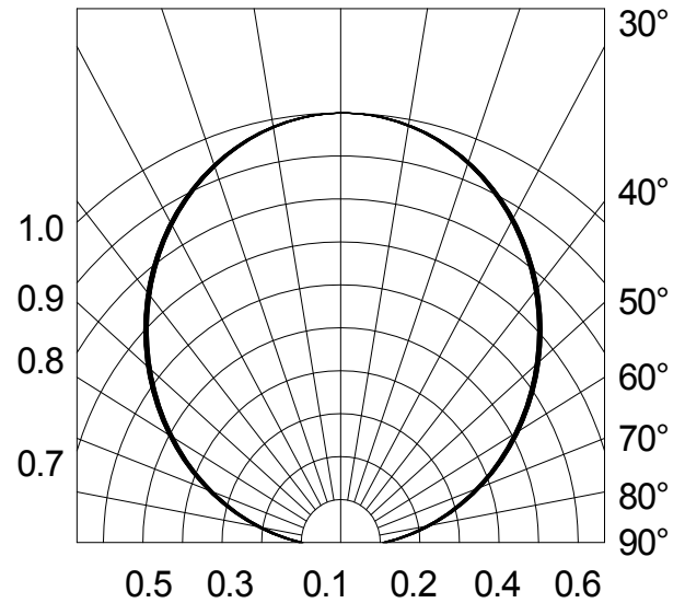
Fig.6-Radiation Diagram Ta=25°C
