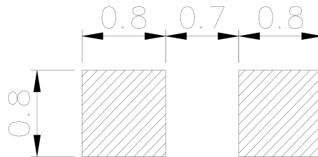
Recommended Solder Pad
