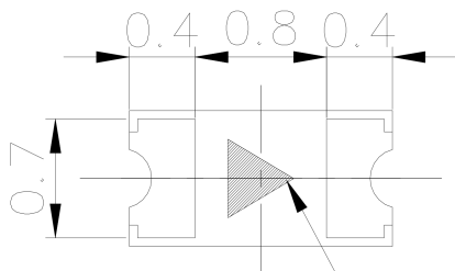
Cathode Mark Bottom View
