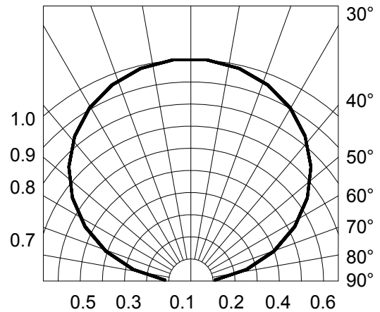
Fig.6-Radiation Diagram
