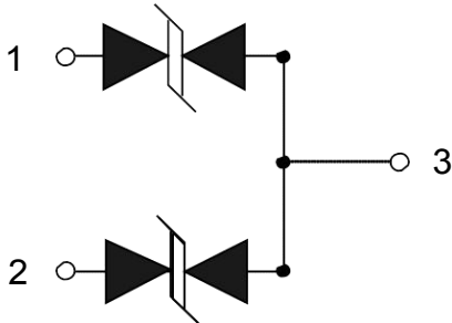
SOT-23 (Top View)
