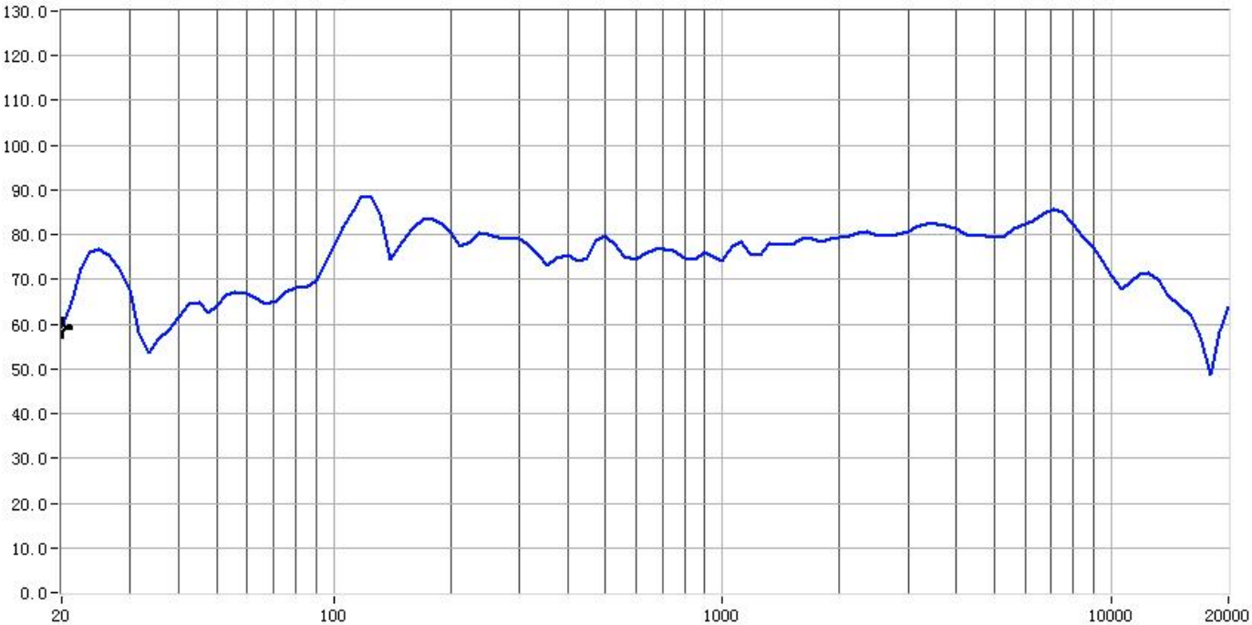
Frequency Response
