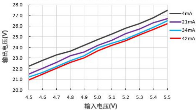
输出电压Vs输入电压@B0524S-1WR2
