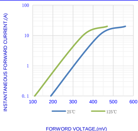
Fig.2-TYPICAL INSTANTANEOUS FORWARD
