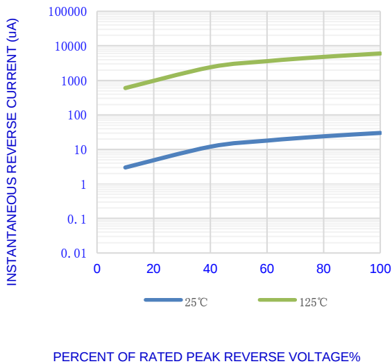
Fig.3-TYPICAL REVERSE CHARACTERISTICS
