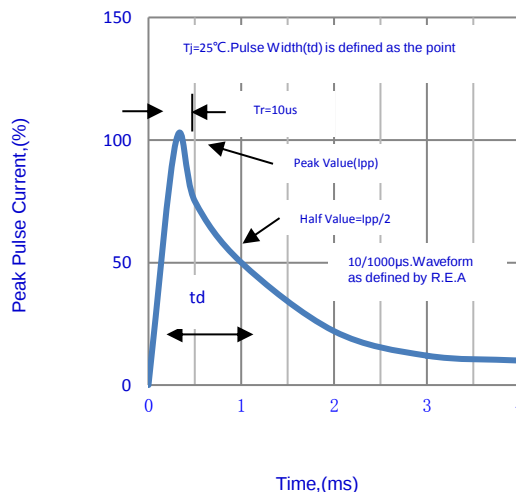
Fig.6-Pulse Waveform
