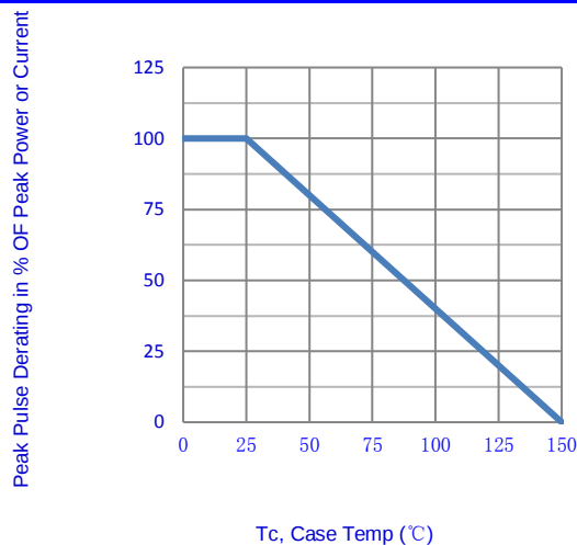
Fig.1-Pulse Derating Curve
