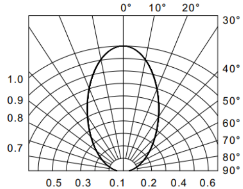
Fig.6-Radiation Diagram T_a=25^{\circ}\text{C}
