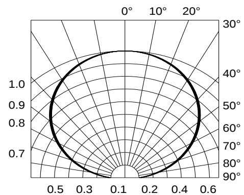
Fig.6-Radiation Diagram T_a=25^{\circ}\text{C}
