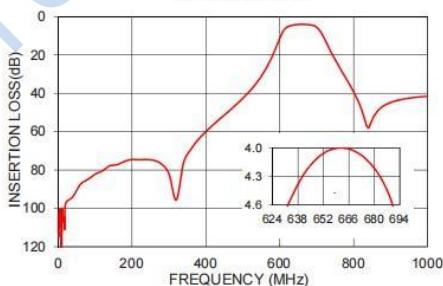
INSERTION LOSS
