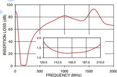
INSERTION LOSS
