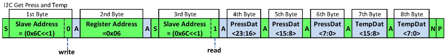
FIGURE 1: SLAVE ADDRESS FOLLOWED BY THREE PRESSURE AND TWO TEMPERATURE BYTES
