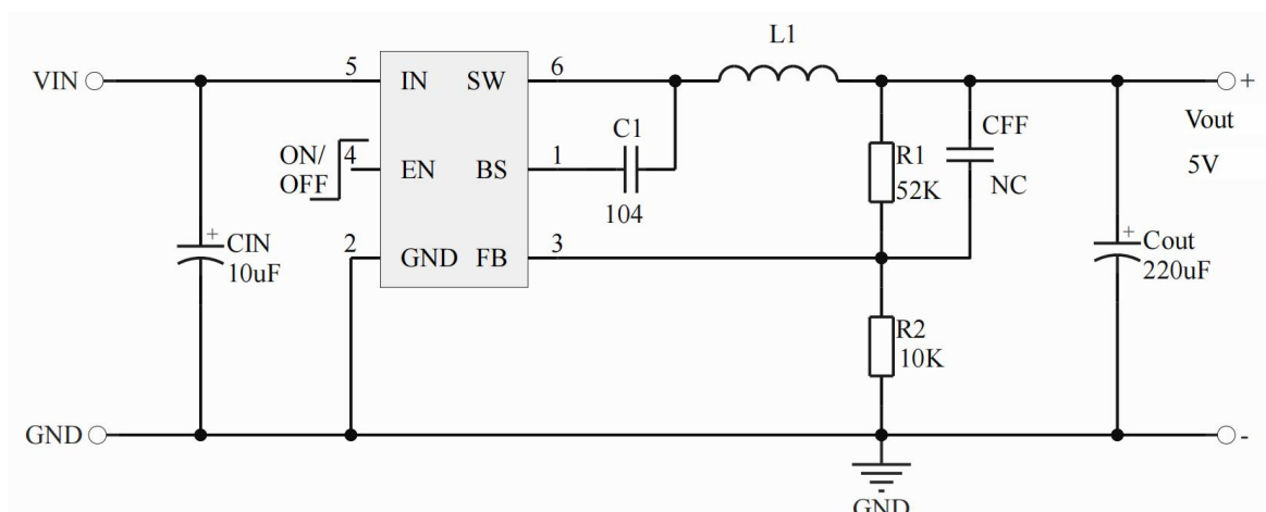
Basic Application Circuit
