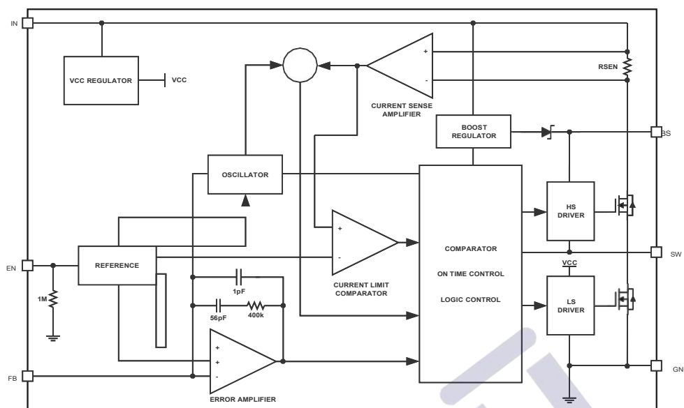
U0138 Block Diagram
