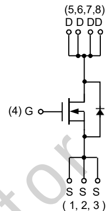
N-Channel MOSFET
