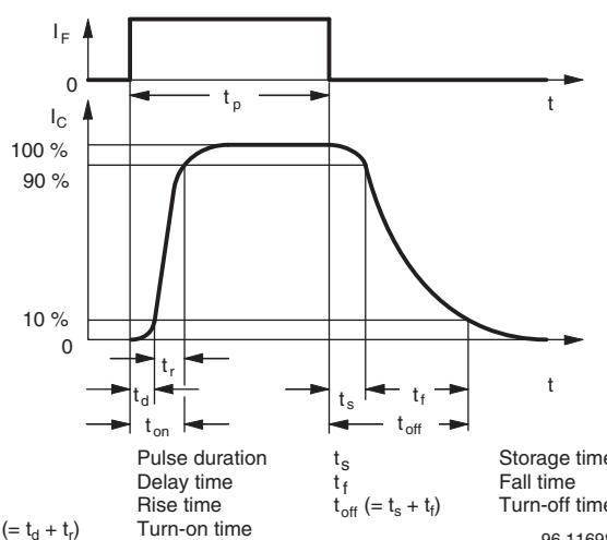
Fig. 3 - Switching Times
