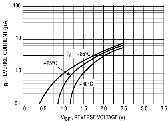
Figure 8. Reverse Characteristics
