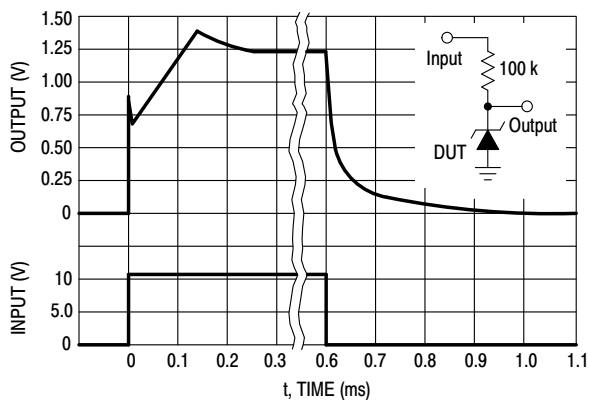
Figure 7. Response Time
