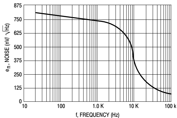
Figure 6. Noise Voltage
