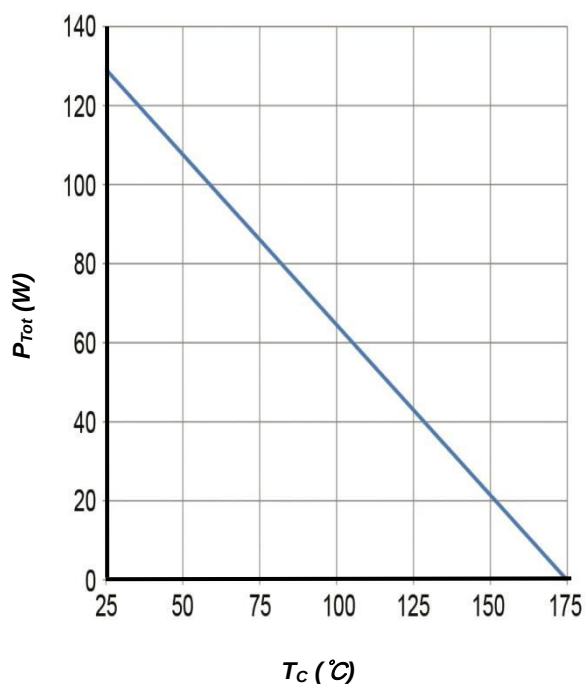
Figure 3. Power Derating
