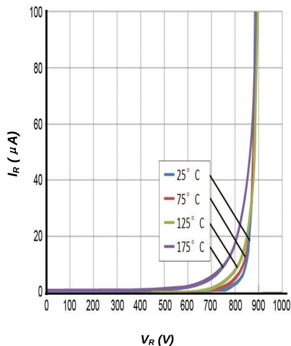
Figure 2. Reverse Characteristics
