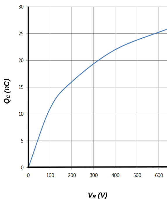
Figure 4. Total Capacitive Charge vs. Reverse Voltage
