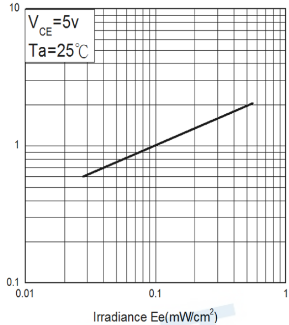
Fig.2 Collector Current vs. Irradiance
