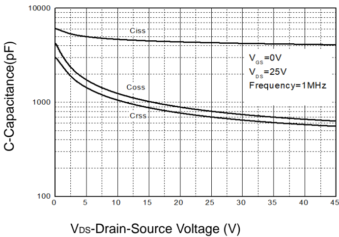
Figure 9: Capacitance Characteristics
