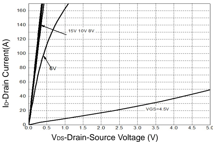
Figure 5: Output Characteristics
