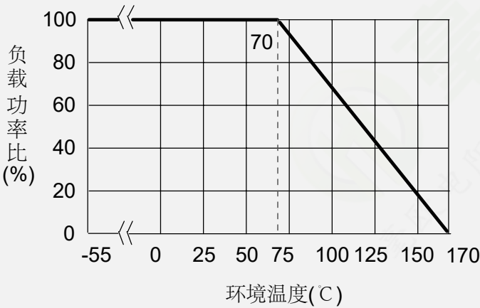
功率曲线 Power Curve
