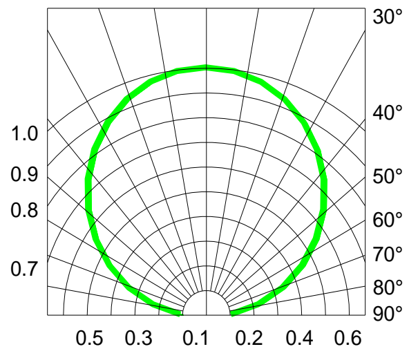
Fig.6-Radiation Diagram T_a=25^\circ\text{C}
