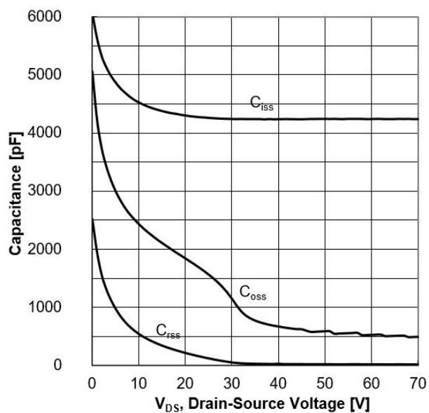
Figure 12. Capacitance Characteristics
