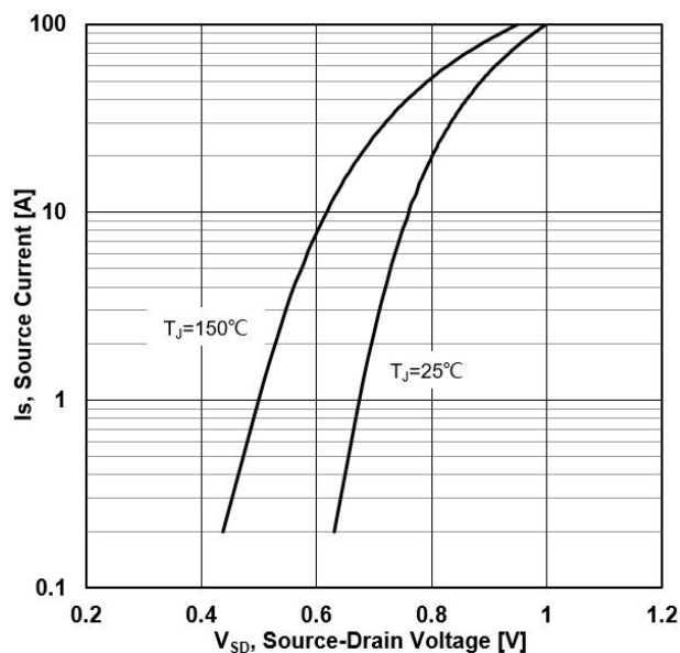
Figure 7. Source-Drain Diode Forward Characteristics
