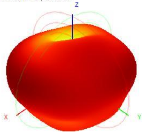
2000.0MHz H+V, Eff: 14.7%
