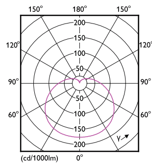
Light Distribution Diagram - ESS LEDBulb 11W E27 3000K 230V 1CT/12 CN
