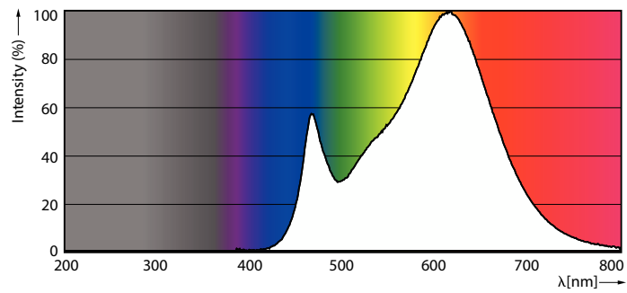
Spectral Power Distribution Colour - ESS LEDBulb 11W E27 3000K 230V 1CT/12 CN
