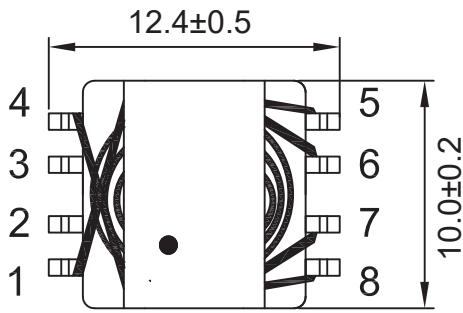
顶视图/Top View
