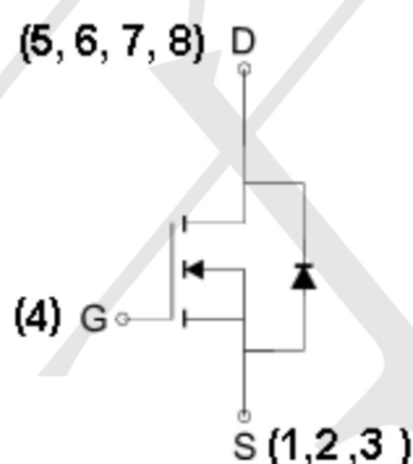
N-Channel MOSFET
