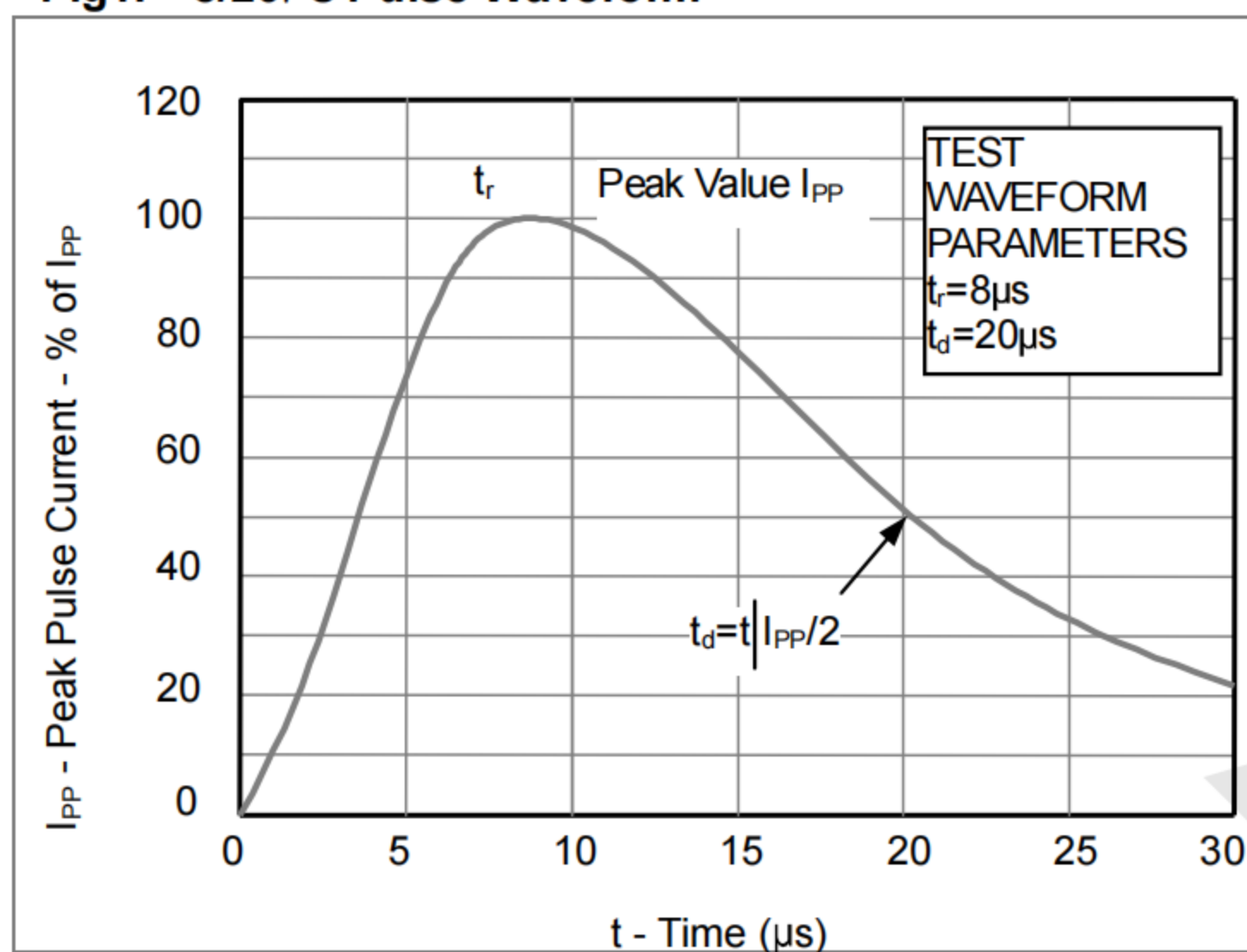
Fig1. 8/20μs Pulse Waveform
