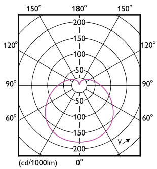
Light Distribution Diagram - ESS LEDBulb 7W E27 3000K 230V 1CT/12 CN
