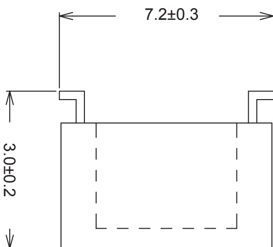
侧视图/Side View
