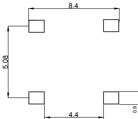
底视图/Bottom View
