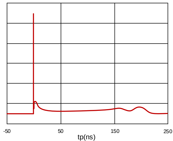
Figure 2: 8kV Contact ESD pulse clamping per IEC61000-4-2
